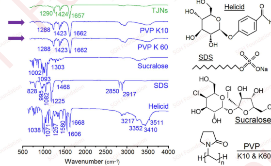
Fig. 7 ATR-FTIR spectra of the TJNs and the five raw materials including PVP K60 and K10, SDS, sucralose, and helicid, and their molecular formula
