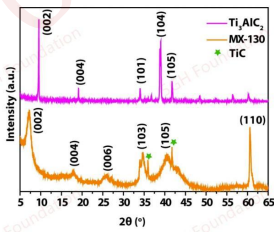
Figure 2. XRD profiles of Ti_3AlC_2 precursor and MX-130 sample showing the formation of Ti_3C_2Tx MXene phase.
