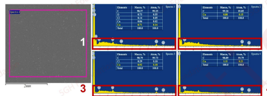
Fig. 3. SEM image and SEM-EDX analysis of oligoCat-Cu (20%) /HDPE surfaces.
