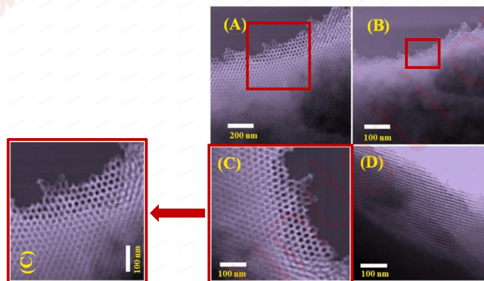
Fig. 2. The TEM images of the mesoporous inorganic silica (A, B) and organic ligand-modified composite adsorbent (C, D) with uniformly arranged pores and ordered structures.
